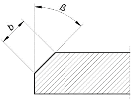
Drawing 1 Bevel dimensions; maximum bevel width depending on the angle
