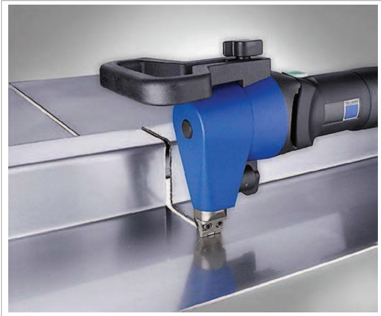
Profile cutting
